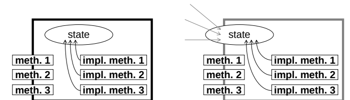
object as implementation of an ADT
